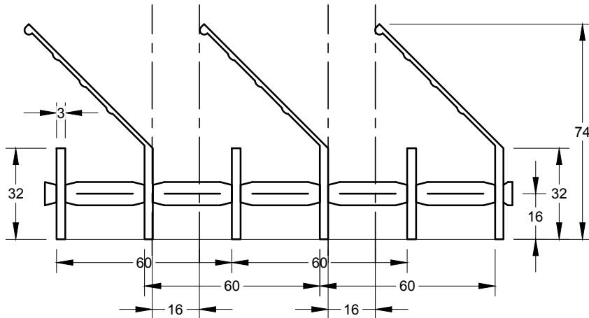
Vertical Panel
