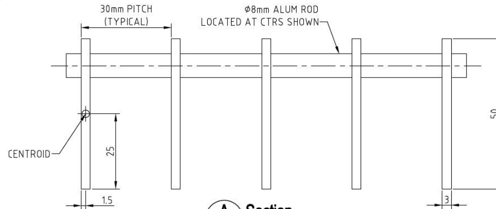
A Section For Horizontal Panel
